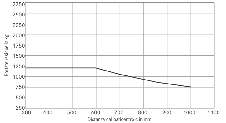
Portate residue FM-X 12/12 N
