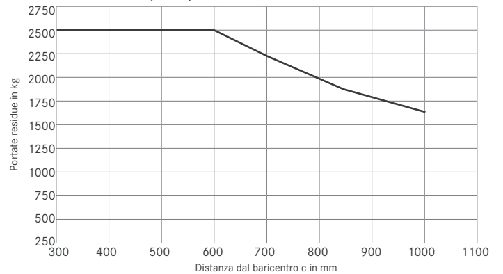
Portate residue FM-X 25/25 W/25 EW
