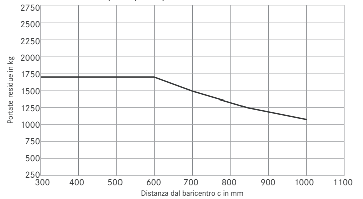
Portate residue FM-X 17/17 N/17 W/17 EW
